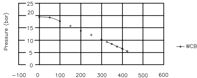
PRESSURE-TEMPERATURE RATING ACCORDING TO ASME B16.34
